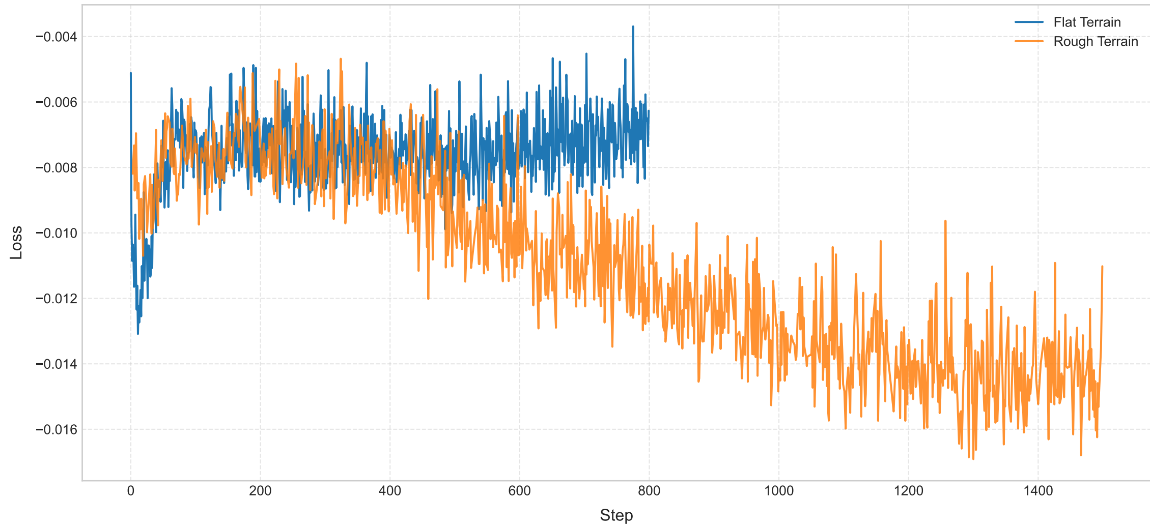
PPO Surrogate Loss (Clipped)
